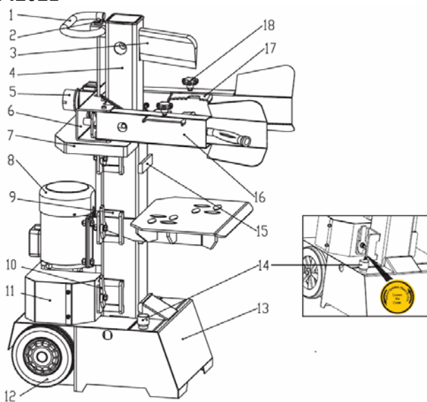
Fig.3 : PREHLS7T/V / 042021
