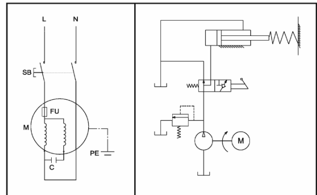
Fig.8b: PREHLS52/5 / 042031
