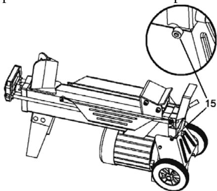
Fig.11: PREHLS52 / 042001 ; PREHLS52/5 / 042031
